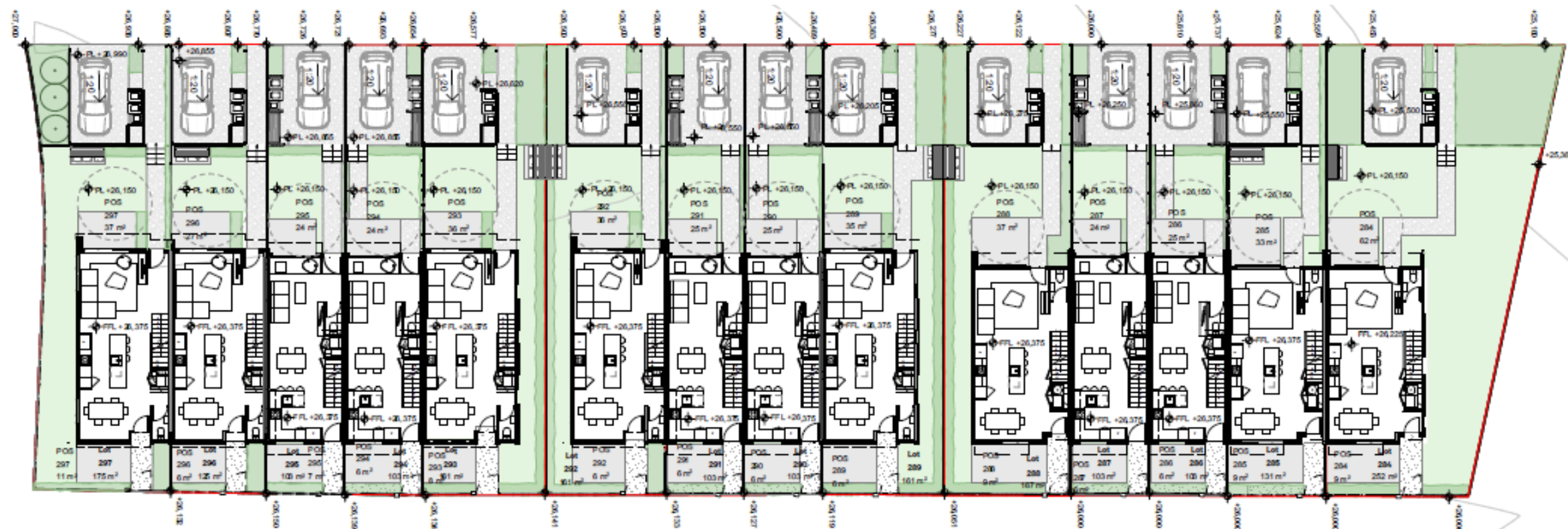
Stage 3a | Block 2, Ground Floor Plan
